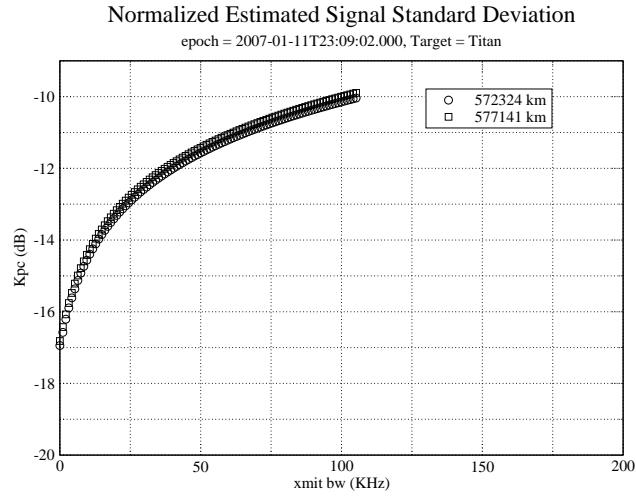
Figure 4: Div f: Normalized estimated signal standard deviation for a disk integrated observation using optimal chirp bandwidth and assuming all the bursts occur at minimum range, and 15 minutes away from minimum range.
