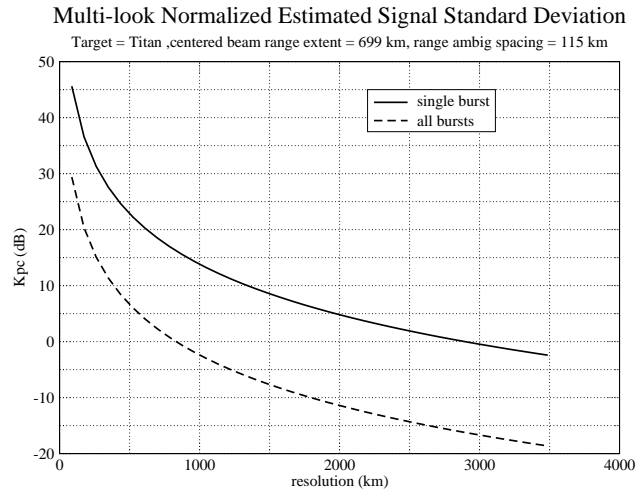
Figure 5: Div f: Normalized estimated signal standard deviation for a range/doppler cell as a function of resolution. Range/doppler resolution elements are both set equal to the specified resolution. Results are shown for a single burst, and for all the bursts in this division. Calculations are performed using the geometry at the start of the division. The presence of ambiguities are not shown.
