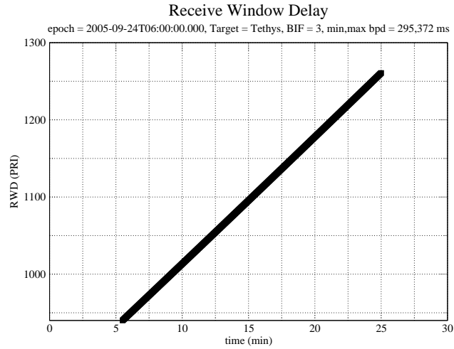
Figure 6: Div D: Inbound scatterometer receive window delay. Subtitle shows the minimum and maximum burst periods that are in principle compatible with the division selected number of bursts in flight.
