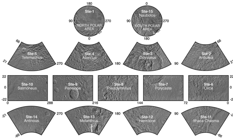
Fig. 6. Fifteen parts of the quadrangle scheme filled with the Tethys.
