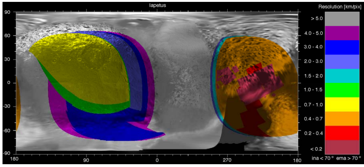
Figure 3c: Total Iapetus coverage planned through the end of Cassini's nominal mission.
