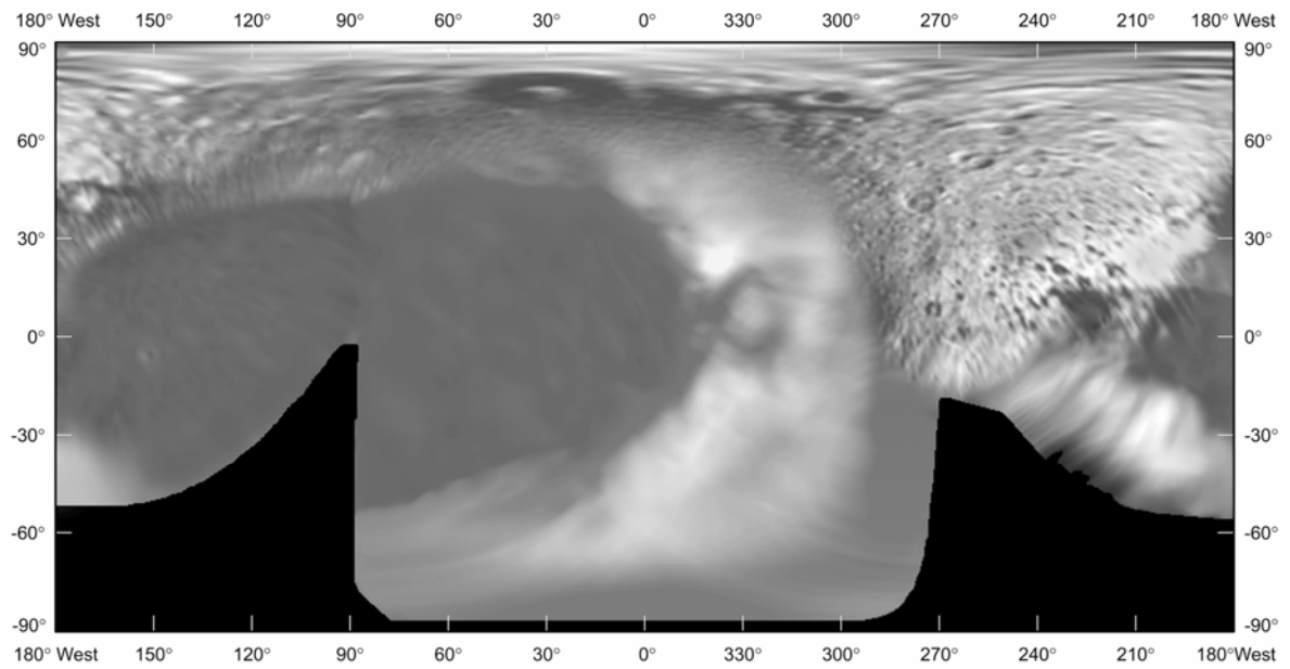
Figure 3a: Iapetus base map generated from Voyager data.
