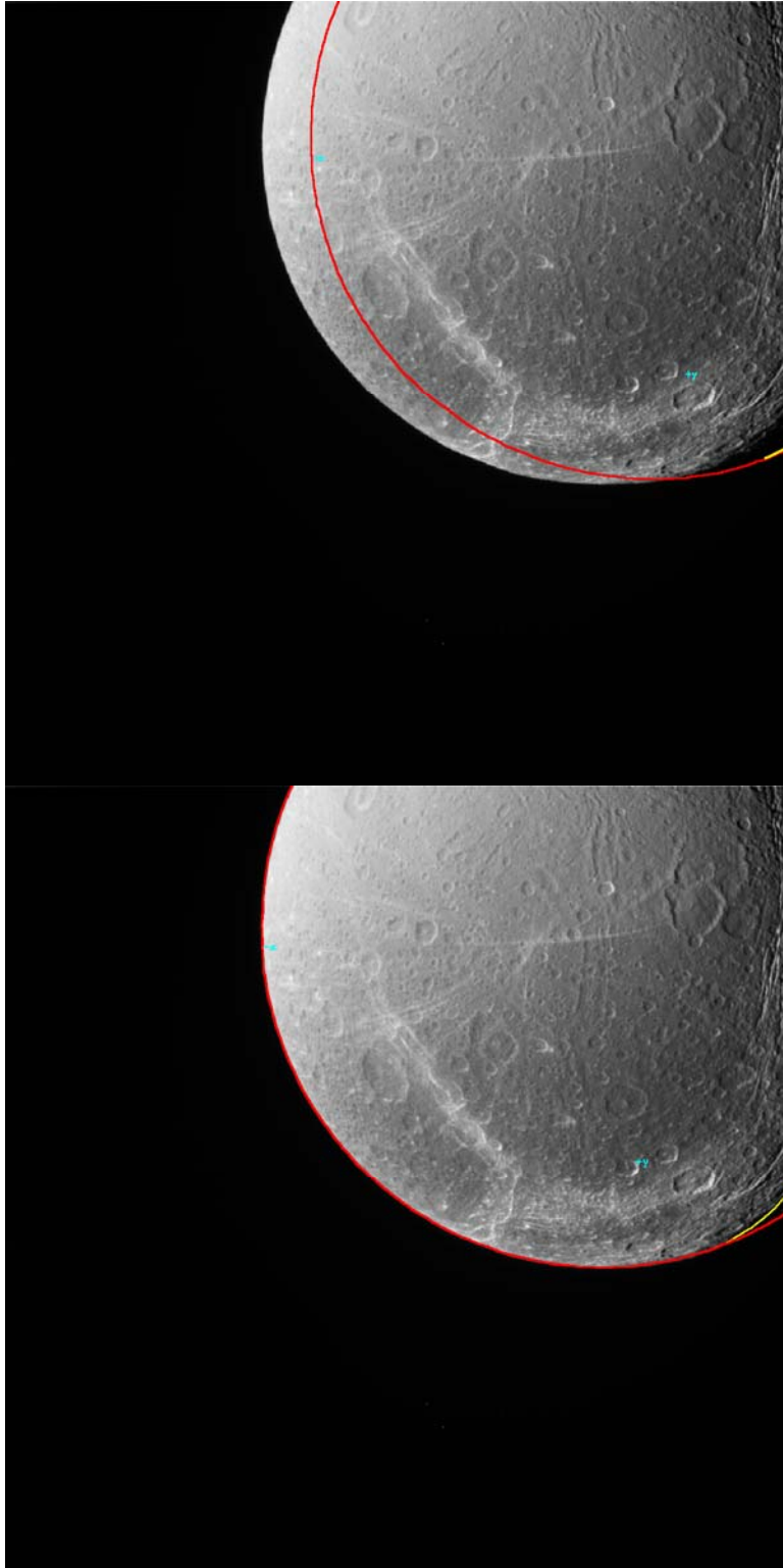
Figure 1: Limb position for satellite Dione, predicted from the SPICE kernel (top) and after interactive limb fitting (bottom)
