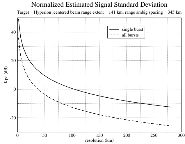
Figure 5: Outbound observation Div D: Normalized estimated signal standard deviation for a range/doppler cell as a function of resolution. Range/doppler resolution elements are both set equal to the specified resolution. Results are shown for a single burst, and for all the bursts in this division. Calculations are performed using the geometry at the start of the division. The presence of ambiguities are not shown.
