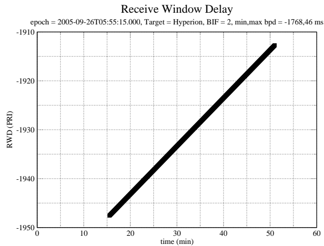
Figure 6: Div D: Inbound scatterometer receive window delay. Subtitle shows the minimum and maximum burst periods that are in principle compatible with the division selected number of bursts in flight.
