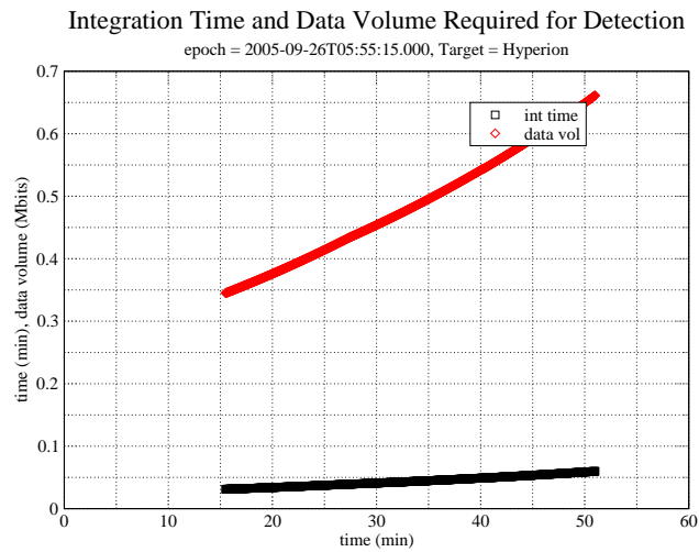
Figure 3: Scatterometry Div D,E: Detection integration time required for a single point detection using optimal chirp bandwidth
